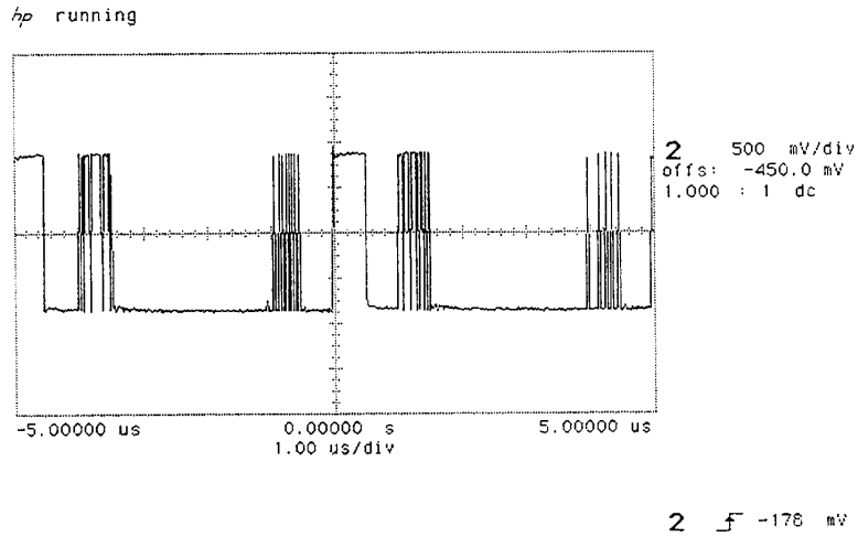
Figure 3-14. Two-Burst Waveform after Autoscale
