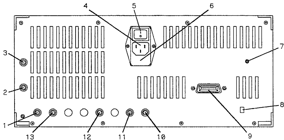
Figure 3-8. Rear Panel Features
