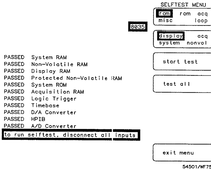
Figure 3-47. Results of Selftest
